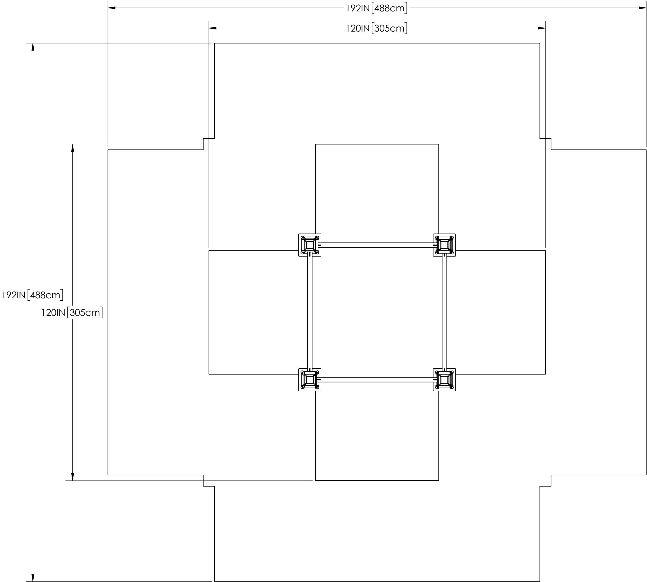
PLAN VIEW
